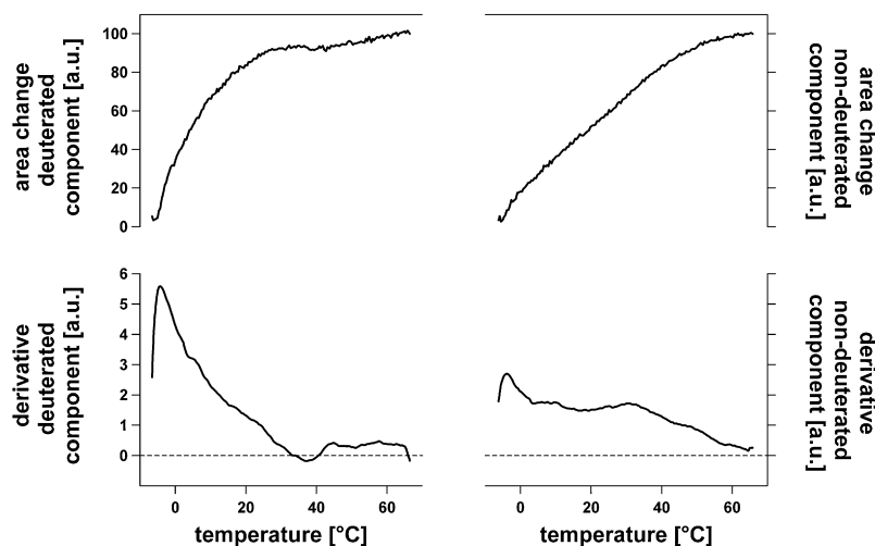
FIGURE 5 Thermal behavior of MLVs composed of dPOPC-d31/pb-cerebrosides 4:1 mol. The values were obtained from area changes of the FTIR spectrum peak at 2920\text{ cm}^{-1} (undeuterated lipid chains) and at 2195\text{ cm}^{-1} (deuterated lipid chains). The figure also shows their corresponding derivatives.
