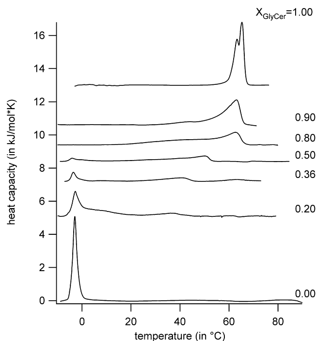
FIGURE 4 DSC thermograms of multilamellar vesicles composed of POPC/pb-cerebroside mixtures at different pb-cerebroside molar ratios.
