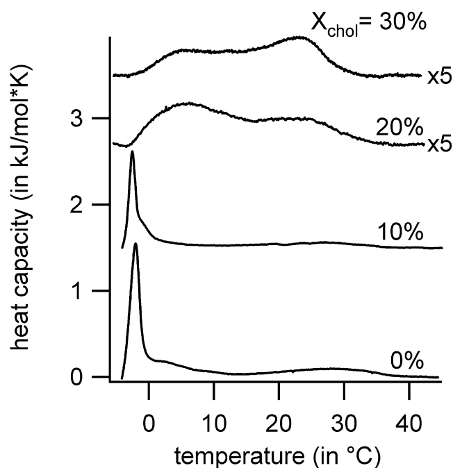
FIGURE 8 DSC thermograms of multilamellar vesicles composed of POPC/pb-cerebroside 4:1 mixture containing different cholesterol concentrations. The two uppermost traces were multiplied by a factor of five for enhancement and clarity.
