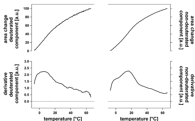
FIGURE 9 Thermal behavior of MLVs composed of dPOPC-d31/pb-cerebroside 4:1 containing 26% cholesterol. The values were obtained from area changes of the FTIR spectrum peak at 2920\text{ cm}^{-1} (undeuterated lipid chains) and at 2195\text{ cm}^{-1} (deuterated lipid chains). The figure also shows their corresponding derivatives.
